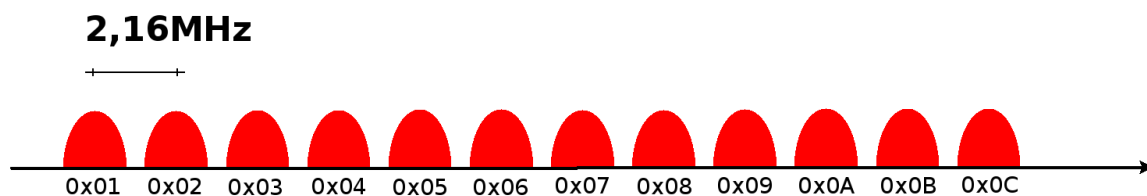
Figure: Channel frequencies in the 900MHz band
