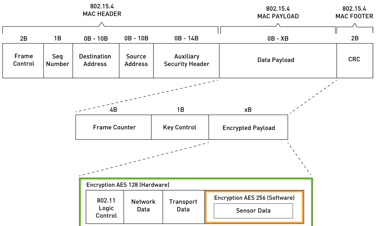
Figure: Waspmote frame structure for communication
