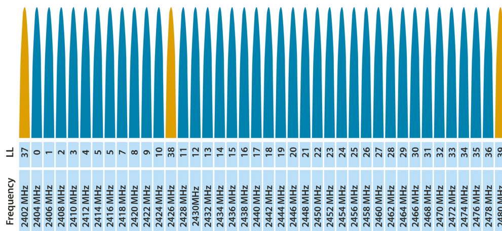
Figure: Channel distribution on the BLE standard
