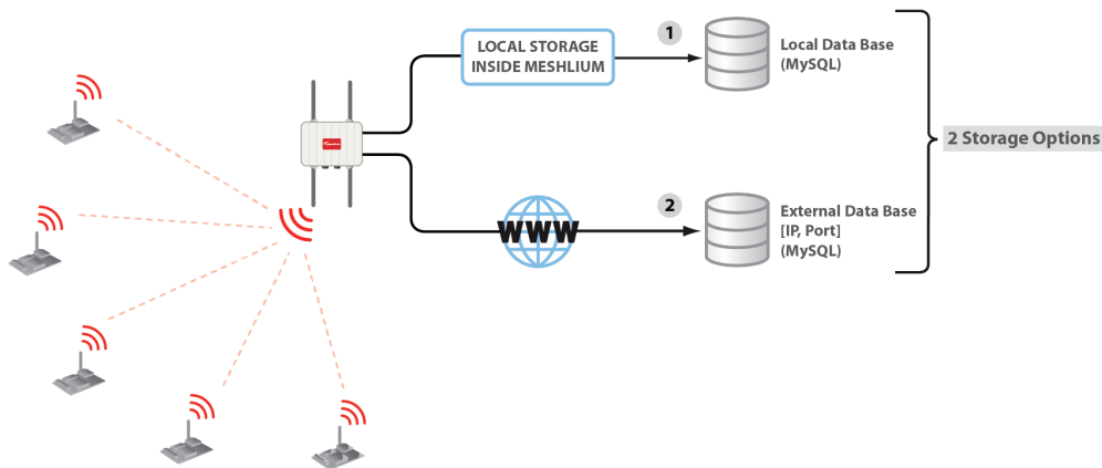
Figure: Meshlium Storage Options
