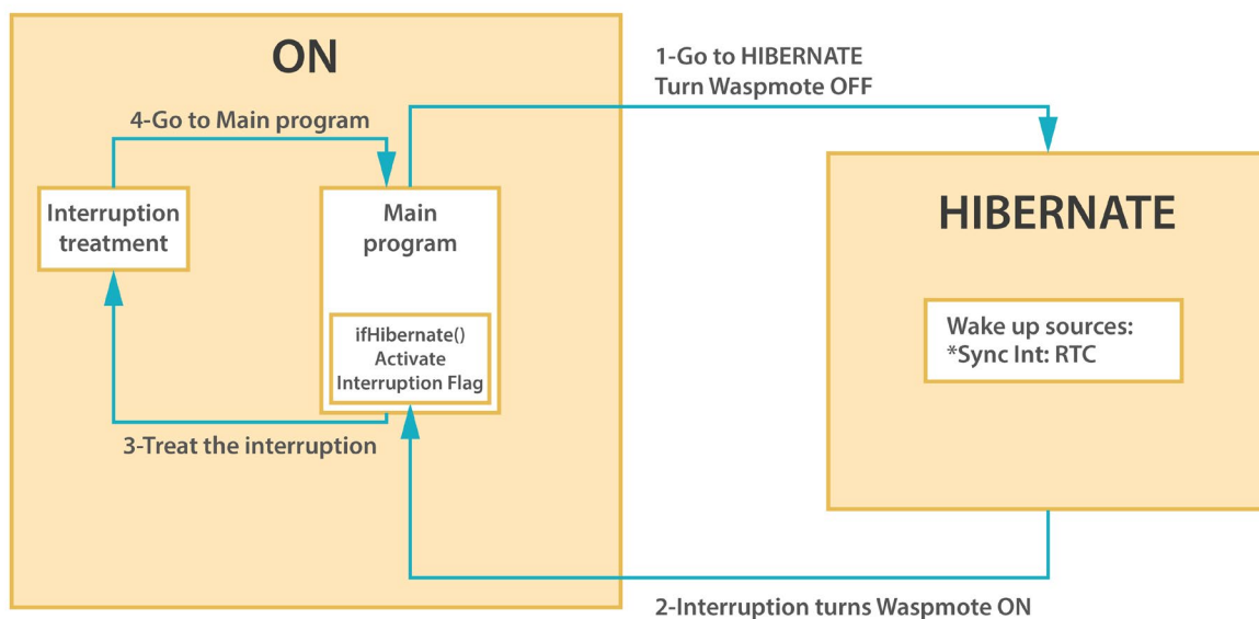
Figure: From ON to Hibernate
