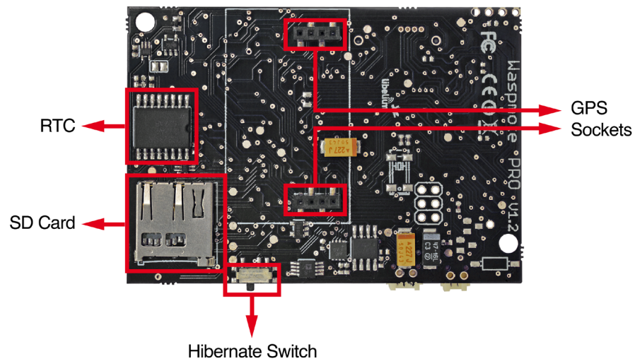
Main Waspote components – Bottom side
