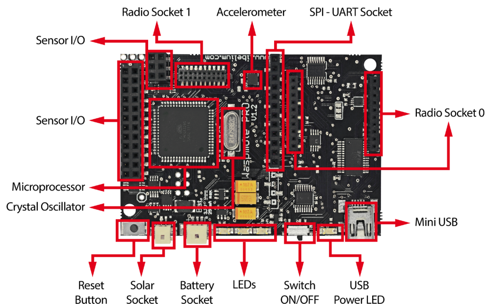
Figure: Main Waspote components – Top side
