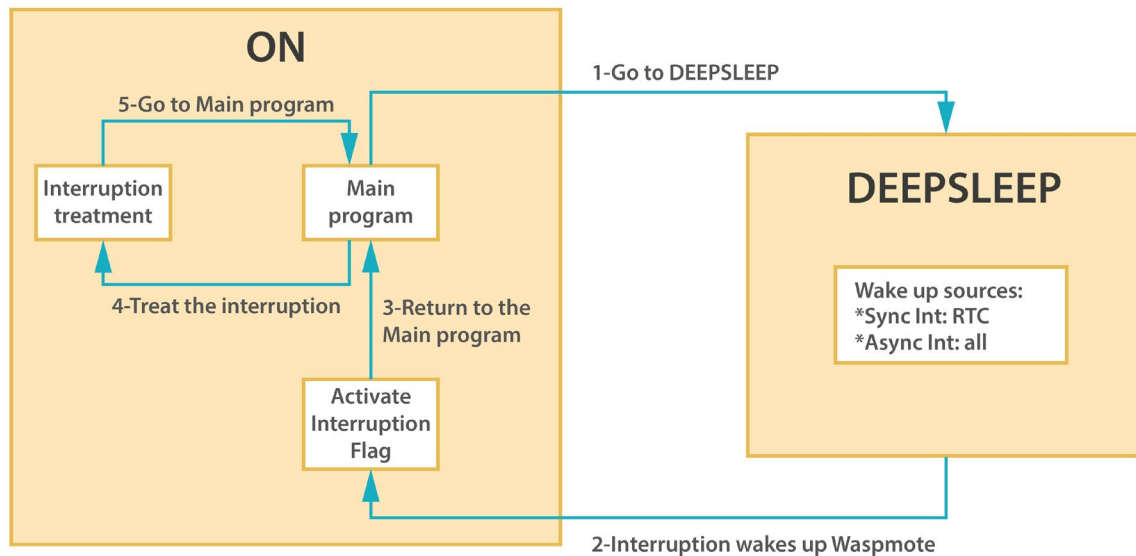
Figure: From ON to Deep Sleep
