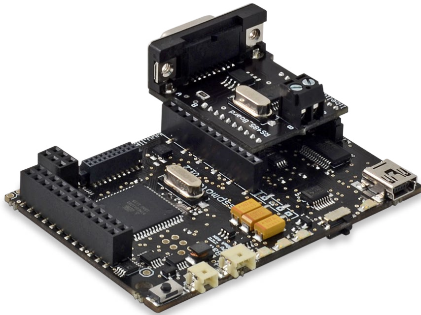
Figure: RS-485 / Modbus module on Wasp mote
