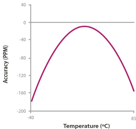
Figure: Uncompensated variation curve
