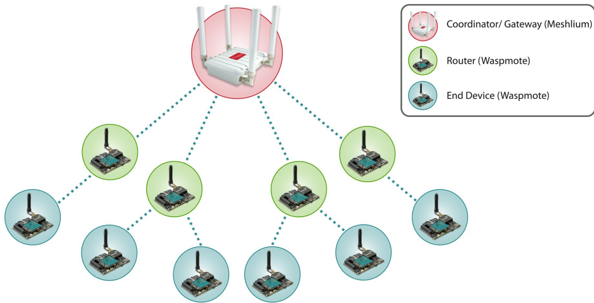
Figure: Tree topology
