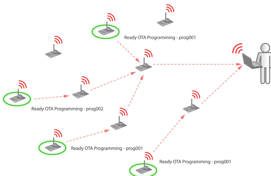
Figure: Wasp motes reply to discovery queries
