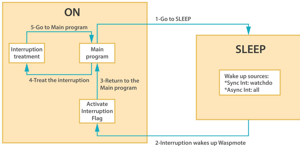
Figure: From ON to Sleep
