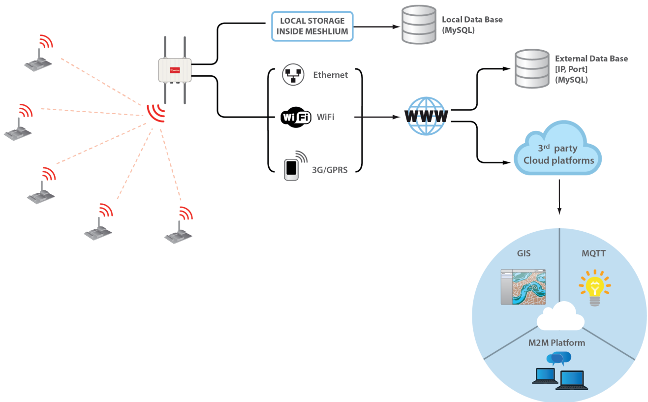
Figure: Meshlium Connection options
