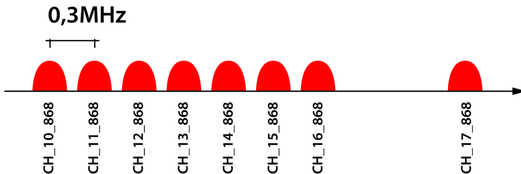
Figure: Channel frequencies in the 868MHz band
