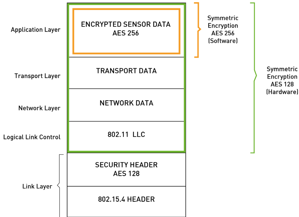
Figure: Waspmote frame on OSI stack for communication
