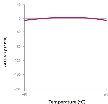
Figure: Compensated variation curve
