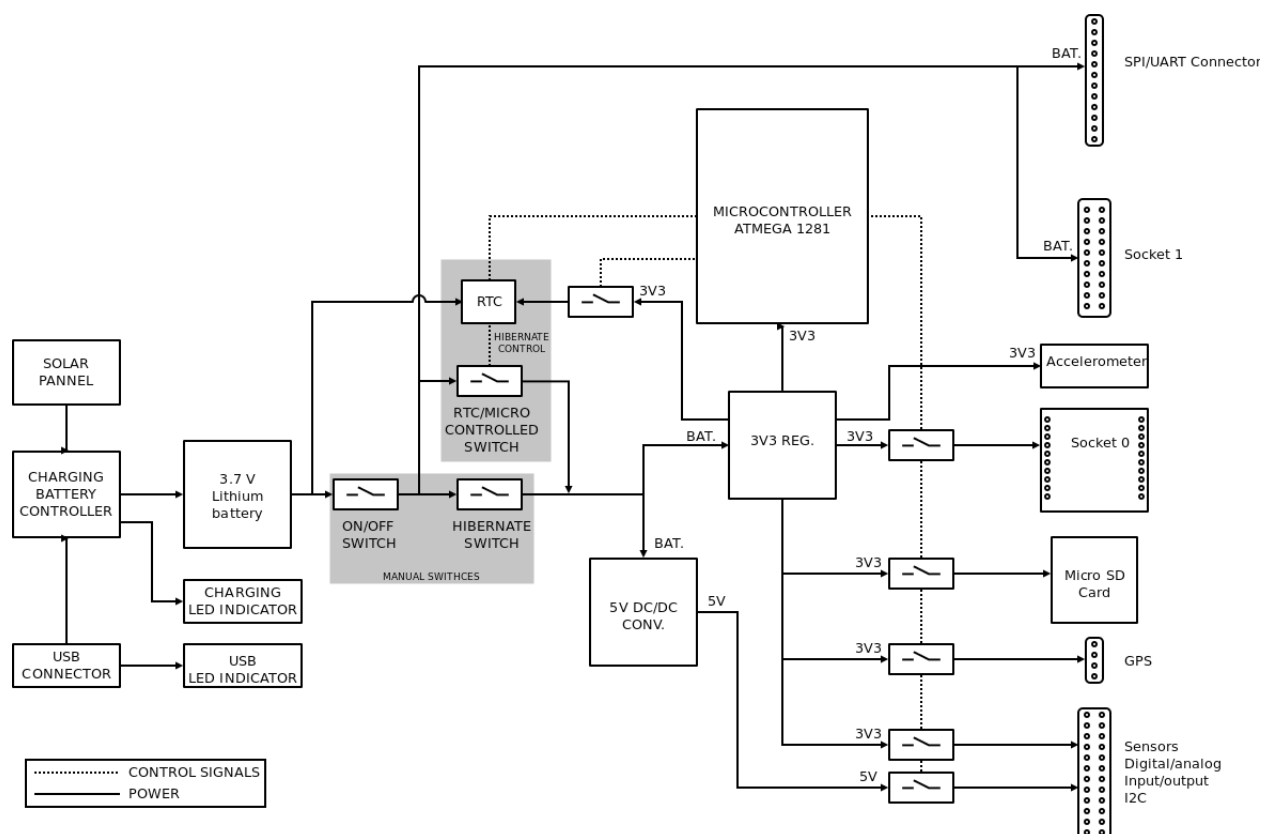
Figure: Waspote block diagrams – Power signals
